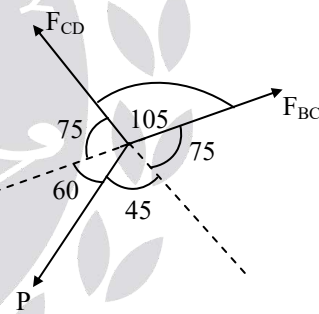
Fig: Free body diagram at 'C'
